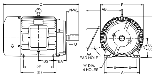
Typical Rigid Base Motor
