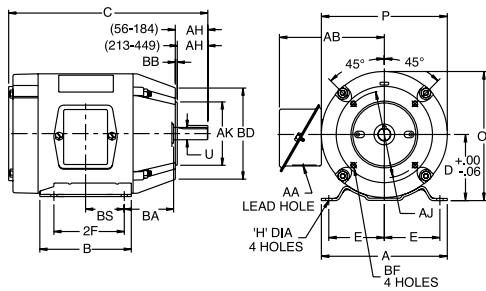
Typical C-Face Motor
